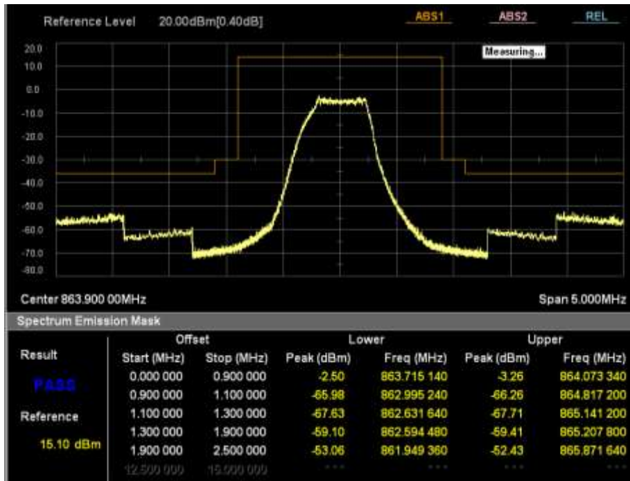
Figure 6-3: Spectrum of a 500 kHz LoRa signal with +14 dBm.
